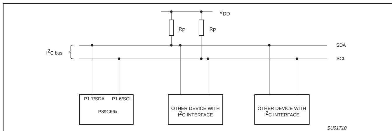
Figure 1. Typical I²C Bus Configuration
