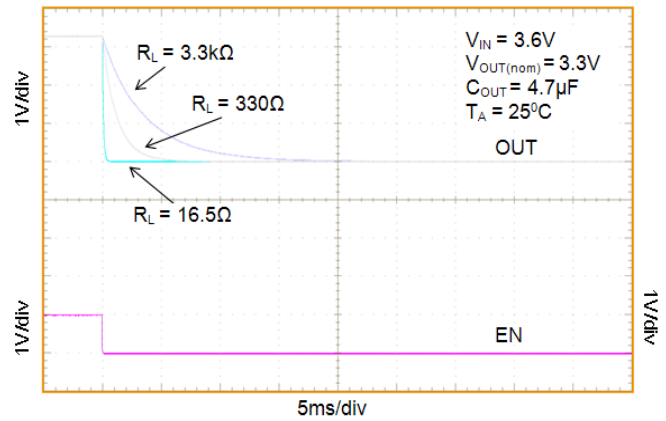
Figure 42. Enable Turn-Off Response, V_{OUT} = 3.3\text{ V} , C_{OUT} = 4.7\text{ }\mu\text{F}
