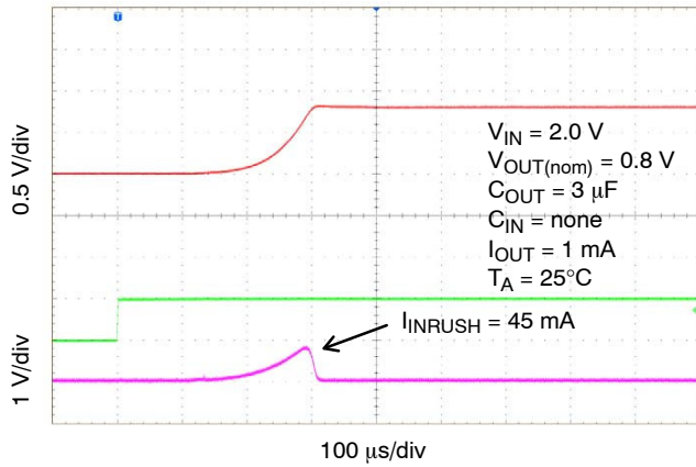
Figure 39. Enable Turn-On Response, V_{OUT} = 0.8\text{ V} , C_{OUT} = 3\text{ }\mu\text{F}
