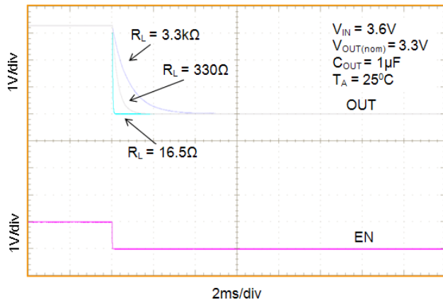
Figure 41. Enable Turn-Off Response, V_{OUT} = 3.3\text{ V} , C_{OUT} = 1\text{ }\mu\text{F}
