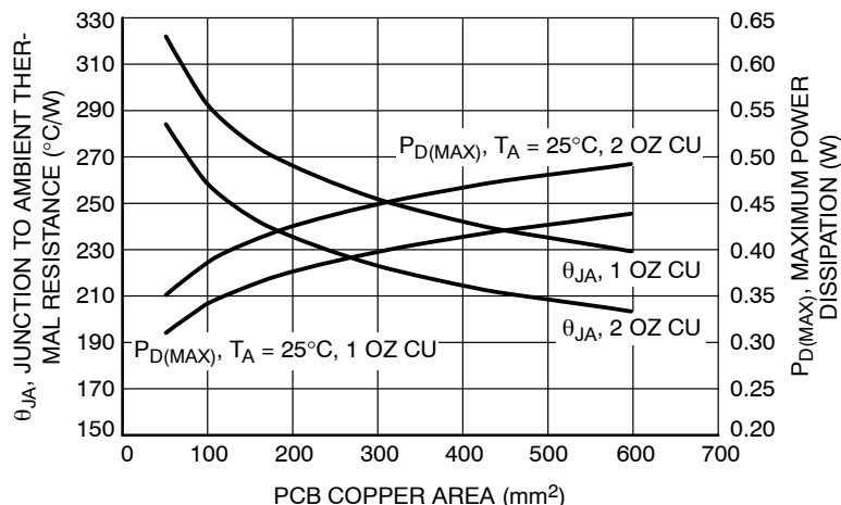
Figure 62. \theta_{JA} and P_{D(\text{MAX})} vs. Copper Area (TSOP5)
