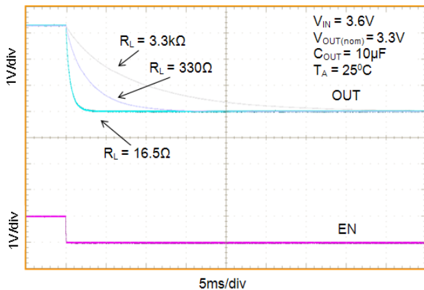
Figure 43. Enable Turn-Off Response, V_{OUT} = 3.3\text{ V} , C_{OUT} = 10\text{ }\mu\text{F}
