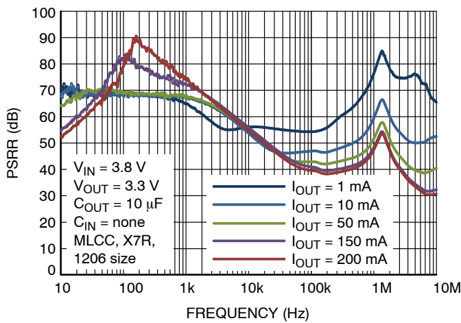
Figure 13. Power Supply Rejection Ratio, V_{OUT} = 3.3\text{ V} , C_{OUT} = 10\text{ }\mu\text{F}
