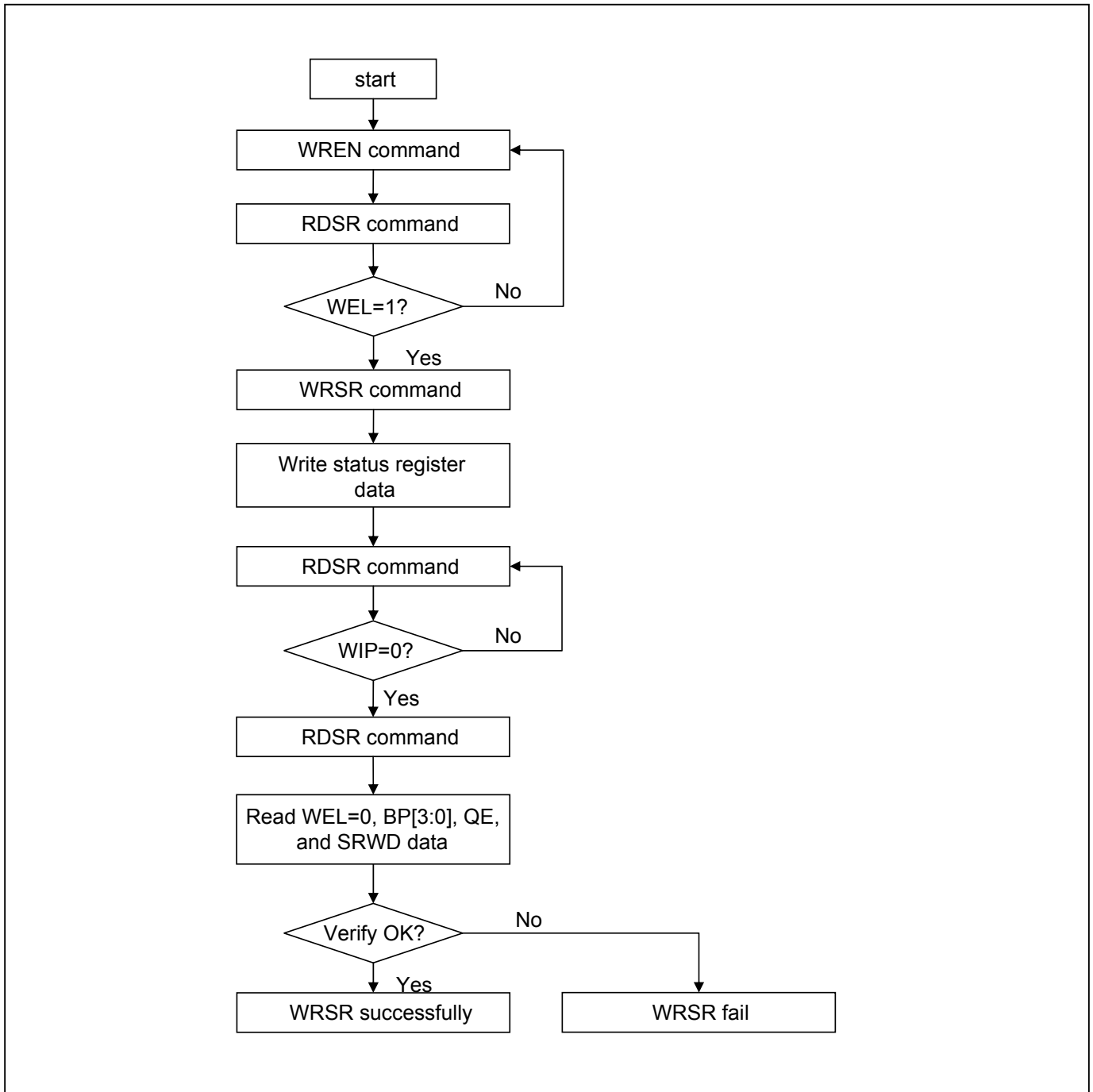
Figure 16. WRSR flow
