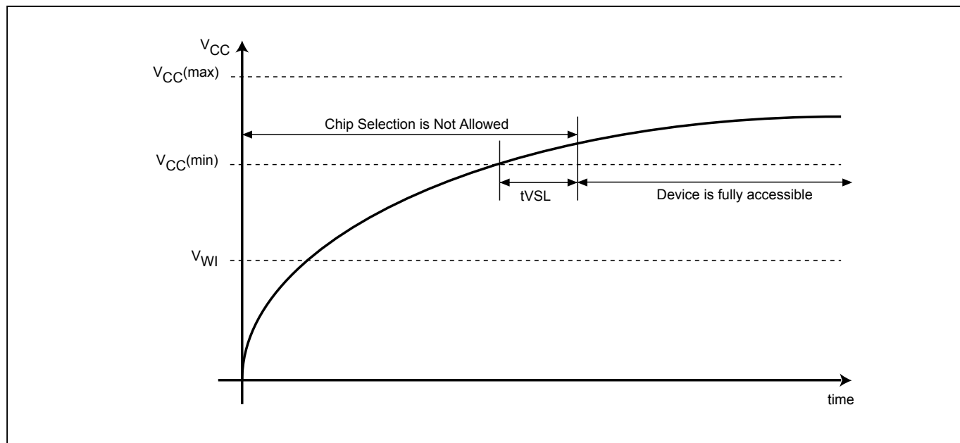
Figure 54. Power-up Timing
