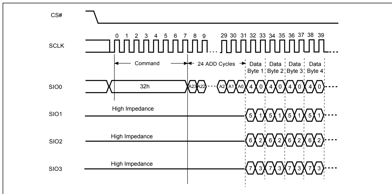
Figure 31. Quad Input Page Program Sequence
