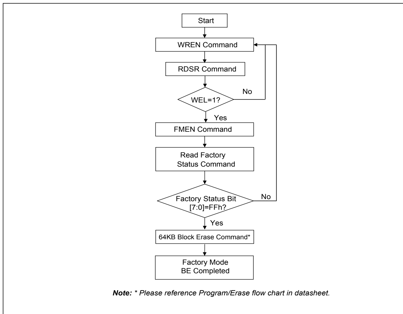
Figure 43. Factory Mode Block Erase Flow
