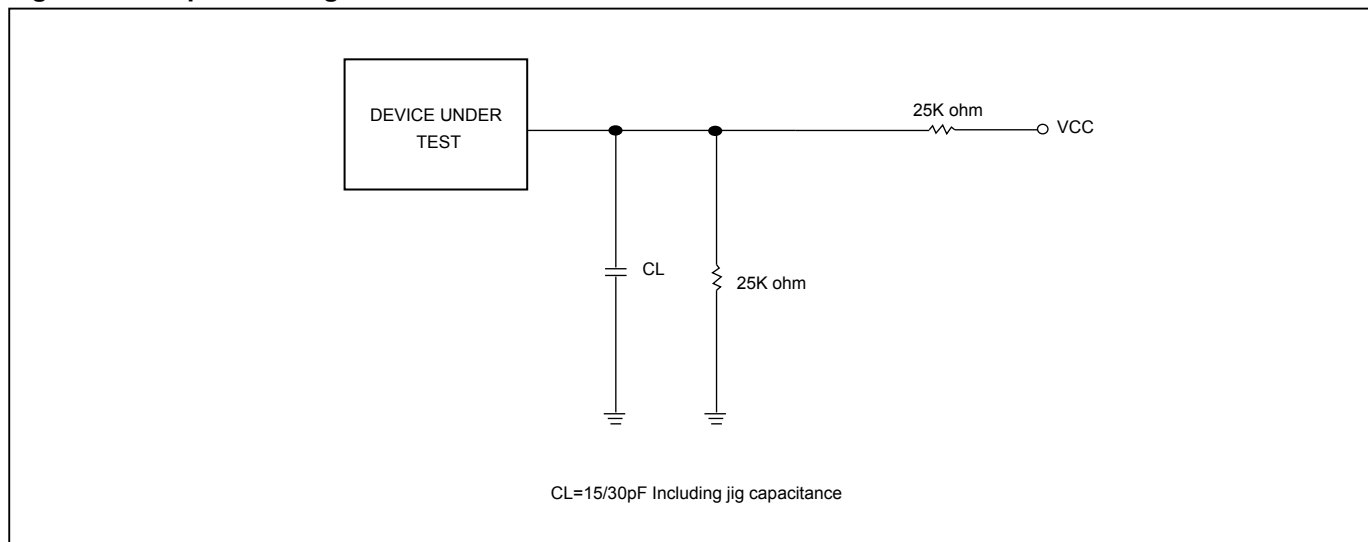
Figure 50. Output Loading
