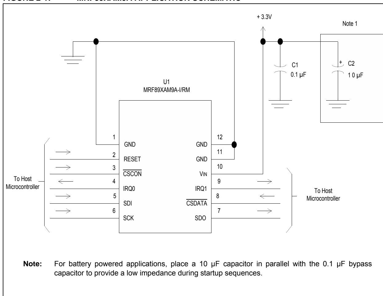
FIGURE 2-1: MRF89XAM9A APPLICATION SCHEMATIC
