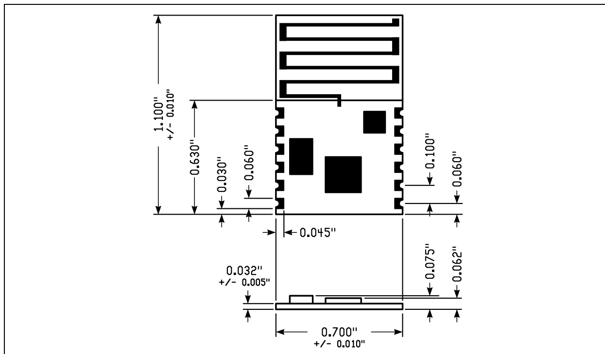
FIGURE 1-3: MODULE DETAILS
