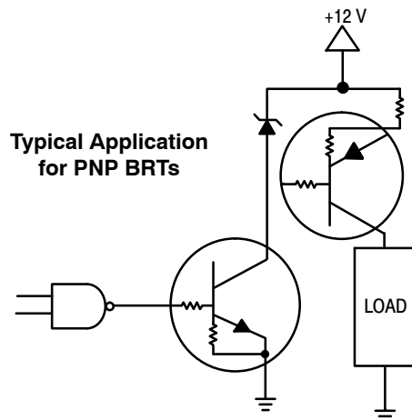
Figure 42. Inexpensive, Unregulated Current Source
