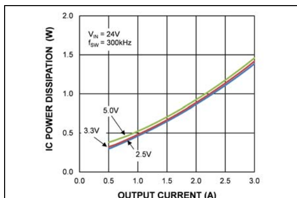
FIGURE 2-32: IC Power Dissipation vs. Output Current (MIC28511-2).
