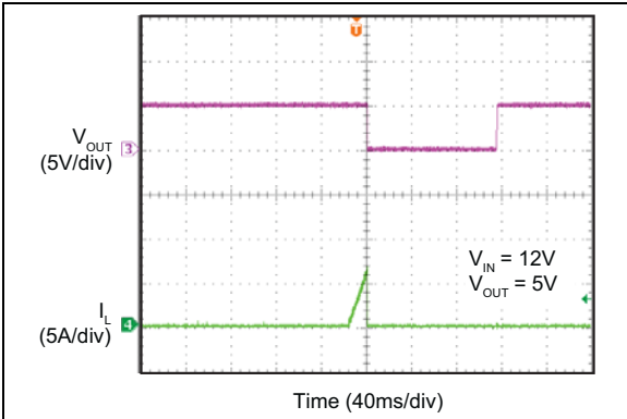
FIGURE 2-46: Output Peak Current-Limit Threshold.
