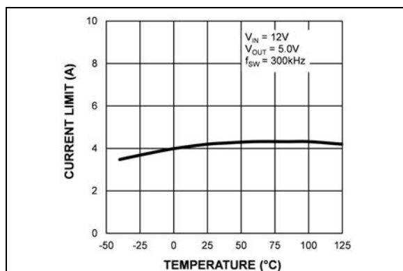
FIGURE 2-7: Output Peak Current Limit vs. Temperature (MIC28511-1).
