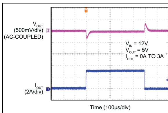
FIGURE 2-55: MIC28511-2 Transient Response.
