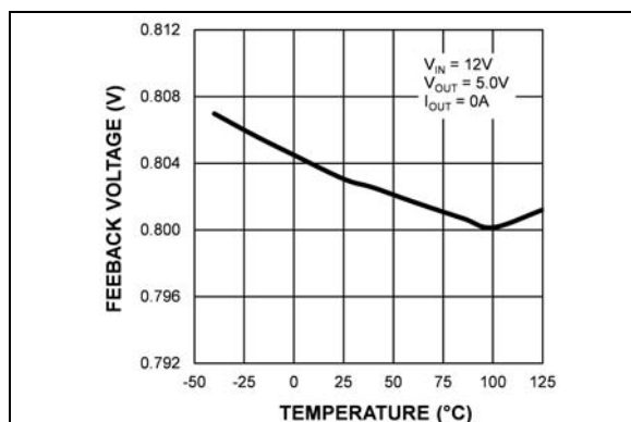
FIGURE 2-8: Feedback Voltage vs. Temperature (MIC28511-1).
