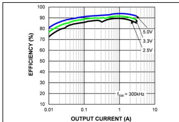
FIGURE 2-11: Efficiency ( V_{IN} = 12V ) vs. Output Current (MIC28511-1).
