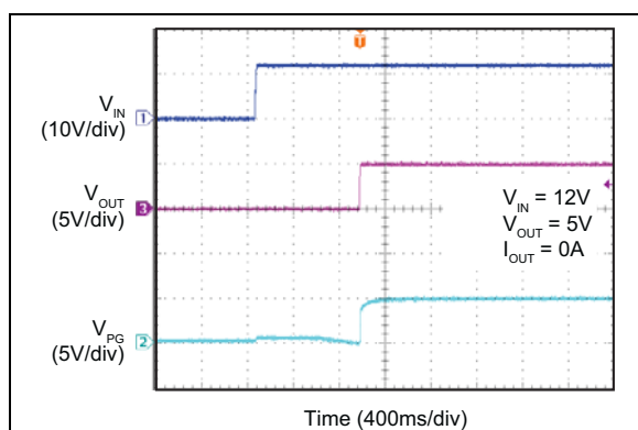
FIGURE 2-57: Power Good at V_{IN} Soft Turn-On.
