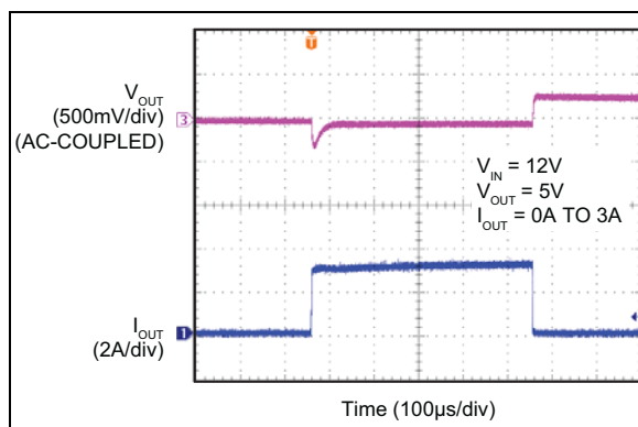
FIGURE 2-56: MIC28511-1 Transient Response.
