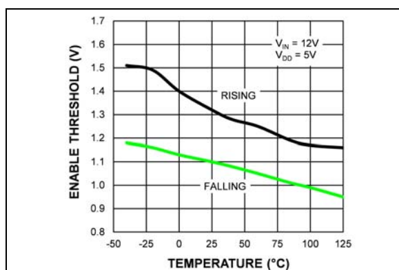
FIGURE 2-9: Enable Threshold vs. Temperature (MIC28511-1).
