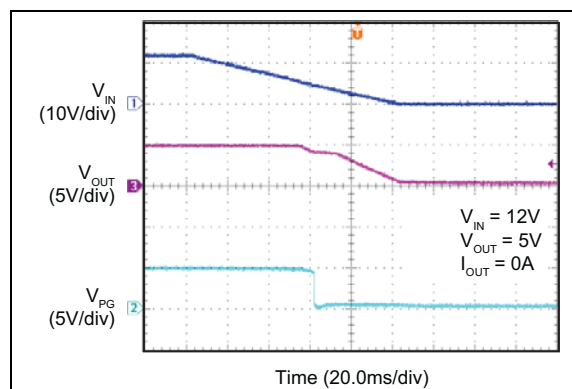
FIGURE 2-58: Power Good at V_{IN} Soft Turn-Off.
