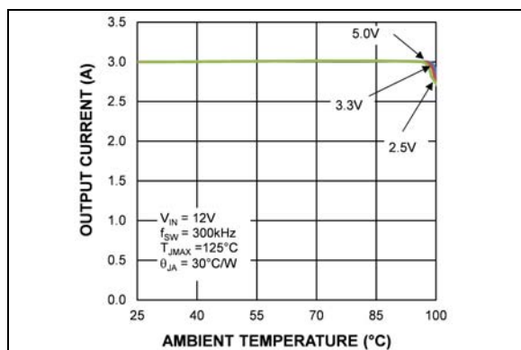
FIGURE 2-31: 12V Input Thermal Derating (MIC28511-2).
