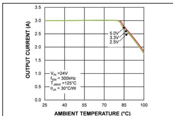
FIGURE 2-19: 24V Input Thermal Derating (MIC28511-1).
