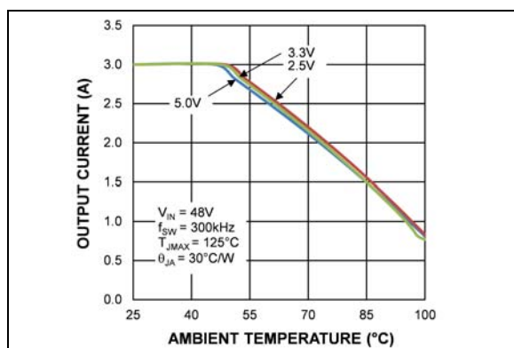
FIGURE 2-20: 48V Input Thermal Derating (MIC28511-1).
