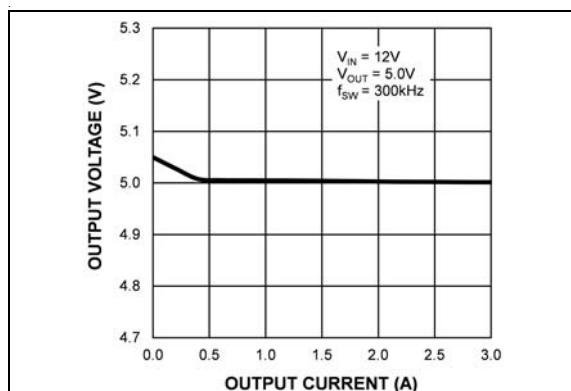
FIGURE 2-10: Output Voltage vs. Output Current (MIC28511-1).
