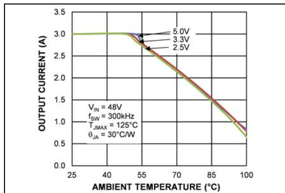
FIGURE 2-35: 48V Input Thermal Derating (MIC28511-2).
