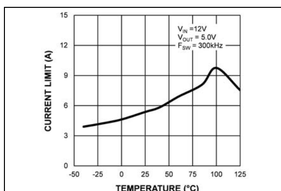
FIGURE 2-24: Output Peak Current Limit vs. Temperature (MIC28511-2).
