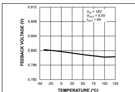
FIGURE 2-23: Feedback Voltage vs. Temperature (MIC28511-2).
