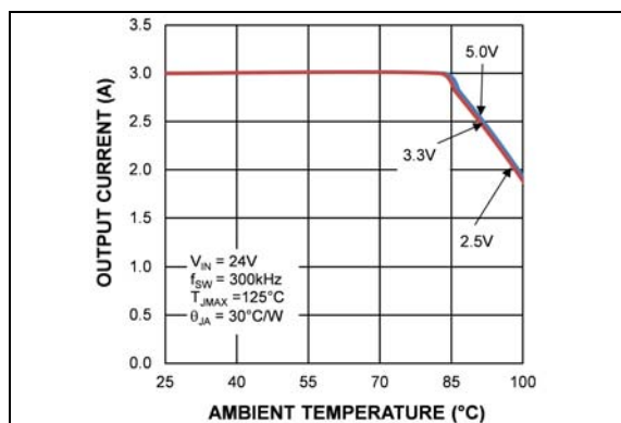
FIGURE 2-34: 24V Input Thermal Derating (MIC28511-2).
