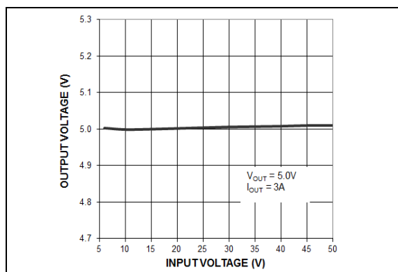
FIGURE 2-22: Output Voltage vs. Input Voltage (MIC28511-2).
