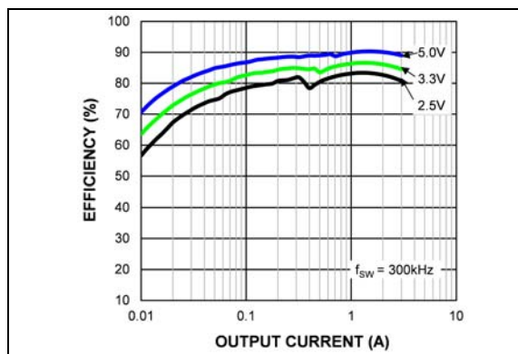
FIGURE 2-12: Efficiency ( V_{IN} = 24V ) vs. Output Current (MIC28511-1).
