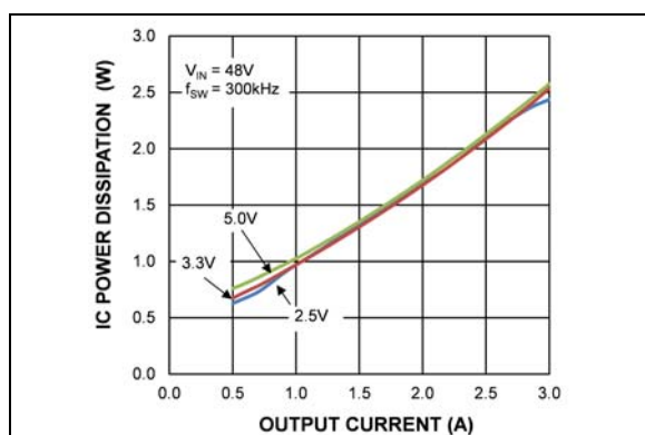
FIGURE 2-33: IC Power Dissipation vs. Output Current (MIC28511-2).
