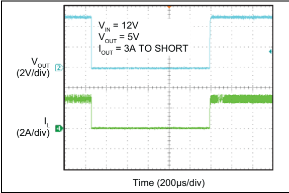
FIGURE 2-48: Output Recovery from Short-Circuit.
