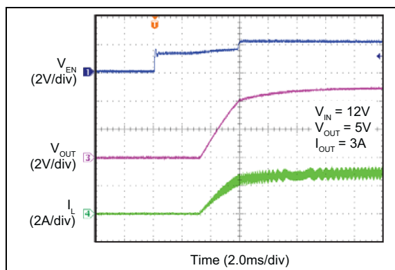
FIGURE 2-36: Enable Turn-On Delay and Rise Time.
