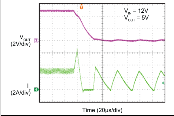
FIGURE 2-47: Short-Circuit.
