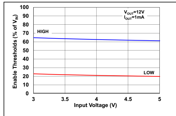
FIGURE 2-14: Enable Threshold vs. Input Voltage.
