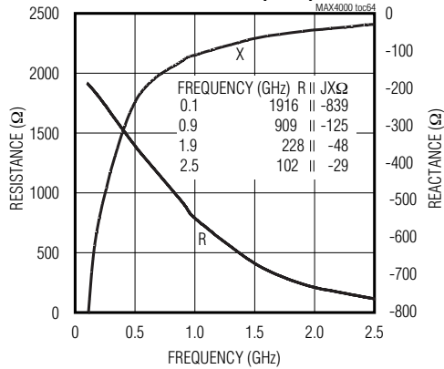
MAX4002 INPUT IMPEDANCE vs. FREQUENCY (UCSP)
