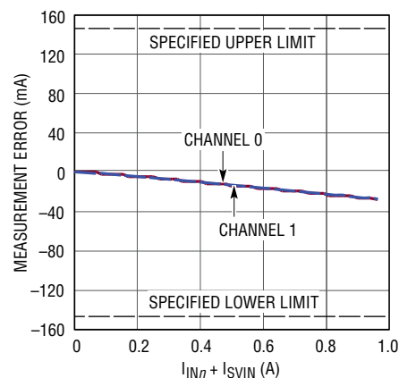
MFR_READ_IIN n (Input Current Readback) Error vs (\text{I}_{\text{VIN}n} + \text{I}_{\text{SVIN}}) , \text{MFR\_PWM\_MODE}_n[0] = 1_b , \text{I}_{\text{OUT}n} Swept from 0\text{A} to 9\text{A} , One Channel at a Time, \text{RUN}_{1-n} = 0\text{V}
