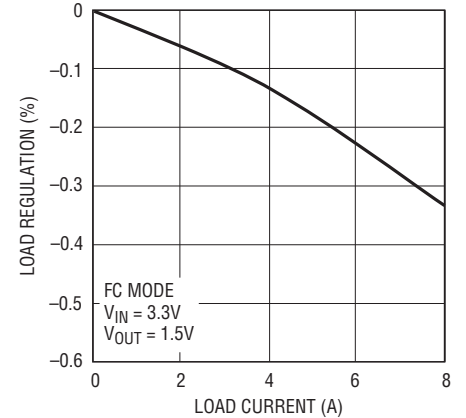
Load Regulation vs Current
