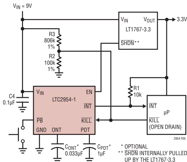
Figure 5. Input Voltage Monitoring with \overline{\text{KILL}} Input
