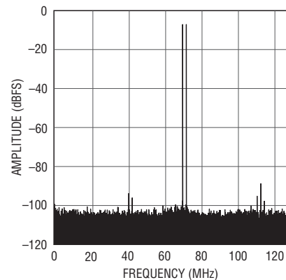
LTC2157-12: 32K Points 2-Tone FFT, f_{IN} = 71\text{MHz} and 69\text{MHz} , 250\text{Mps}
