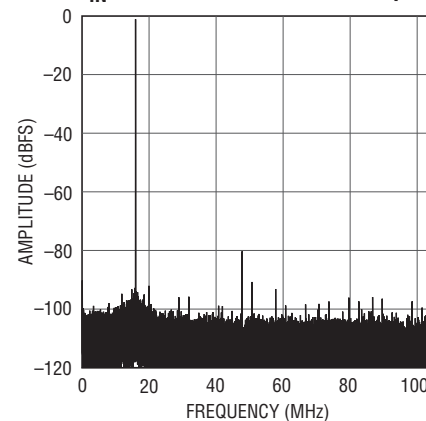
LTC2156-12: 32K Point FFT, f_{IN} = 227\text{MHz} , -1dBFS, 210MSPs
