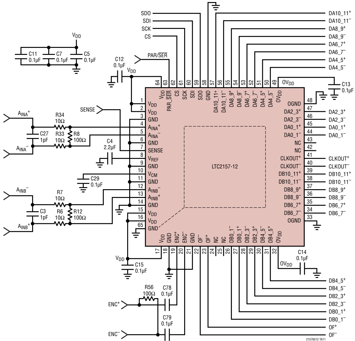
LTC2157-12 Schematic
