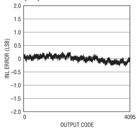
LTC2156-12: Integral Nonlinearity (INL)
