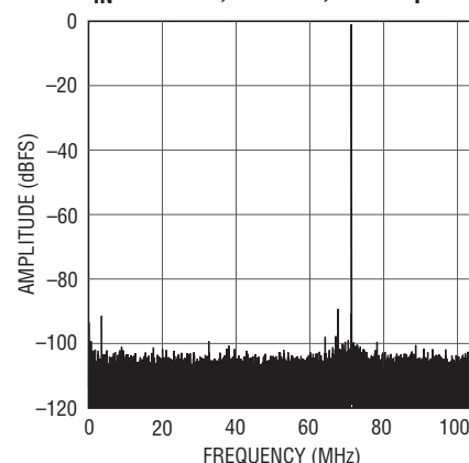
LTC2156-12: 32K Point FFT, f_{IN} = 71\text{MHz} , -1dBFS, 210MSPs
