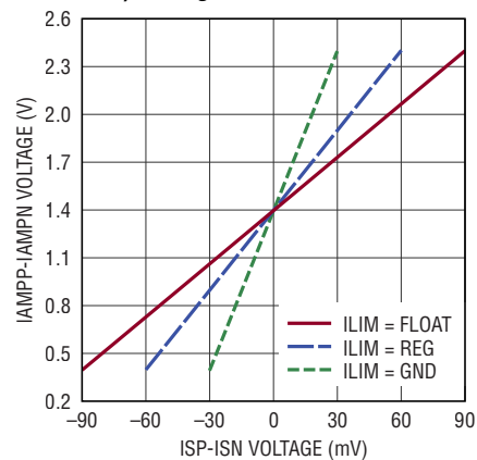
I AMP P-I AMP N Voltage vs (I SP -I SN ) Voltage
