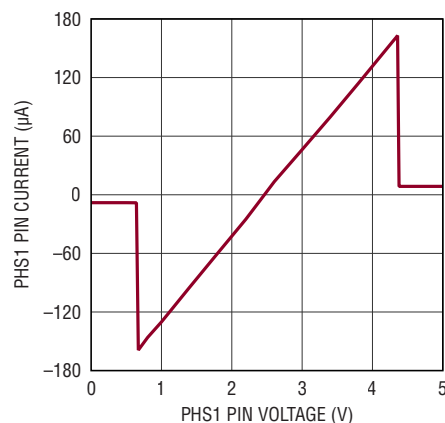
PHS1 Pin Current
