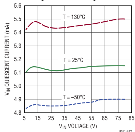
V IN Quiescent Current vs V IN Voltage, Not Switching
