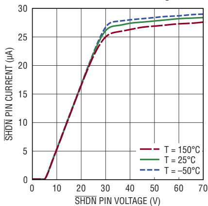
SHDN Pin Current vs Voltage
