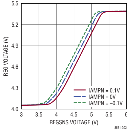
REG Voltage vs REGSNS Voltage
