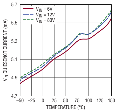
V IN Quiescent Current vs Temperature, Not Switching
