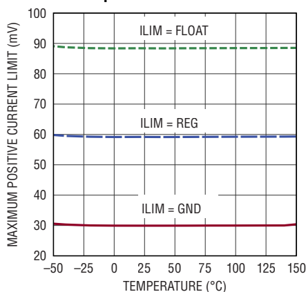
Maximum Positive Current Limit vs Temperature
