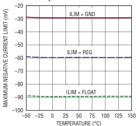
Maximum Negative Current Limit vs Temperature
