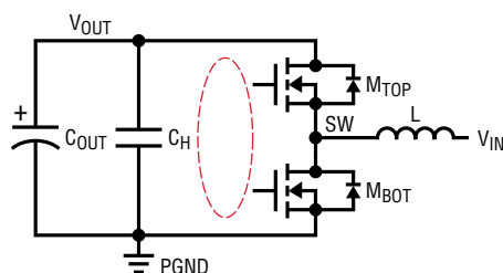
a) High di/dt Loop
