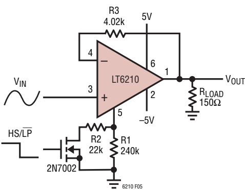
Figure 5. Line Driver with Low Power Mode
