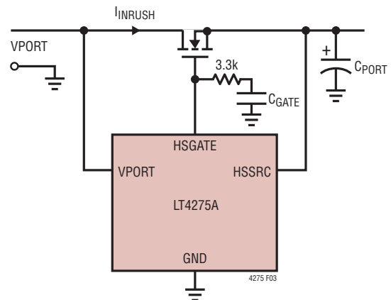
Figure 3. Programming I INRUSH
