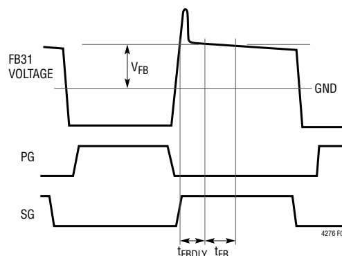
Figure 13: Feedback Amplifier Timing Diagram
