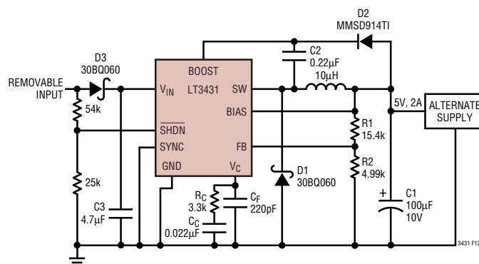
Figure 12. Dual Source Supply with 25μA Reverse Leakage
