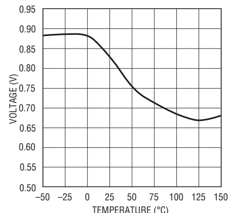
VC Switching Threshold vs Temperature
