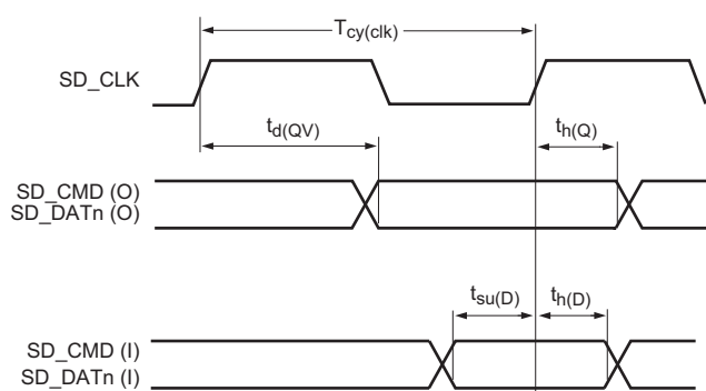
Fig 39. SD/MMC timing
