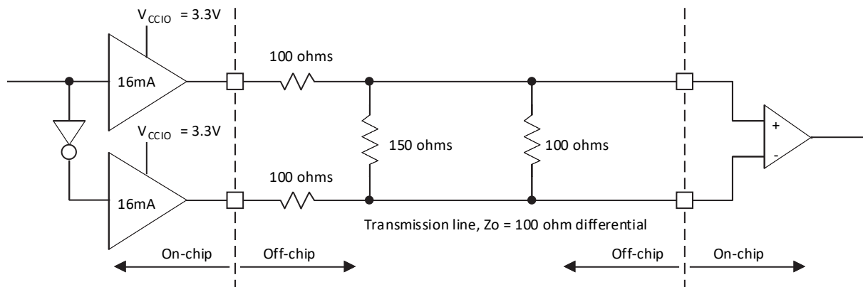
Figure 3.25. Differential LVPECL
