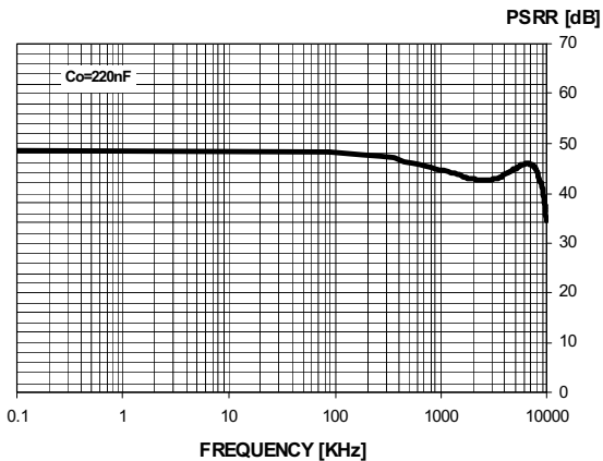
Figure 13. PSRR
