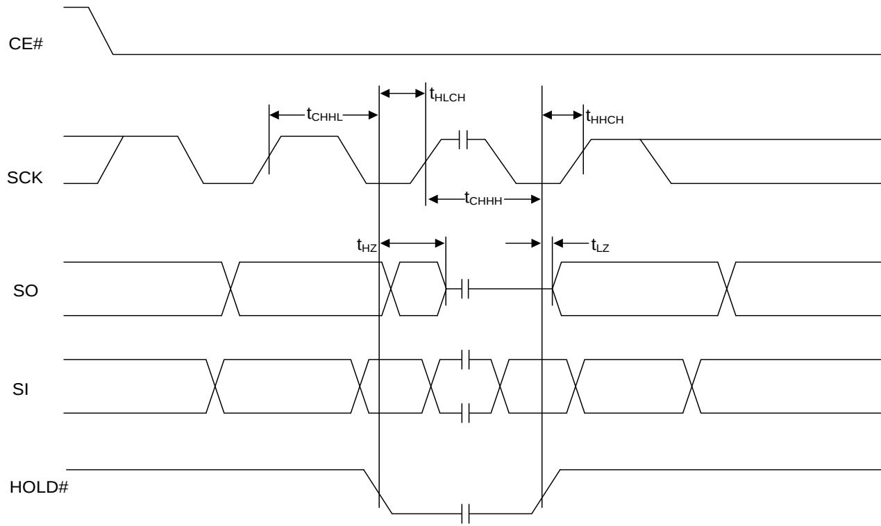
Figure 9.4 HOLD TIMING
