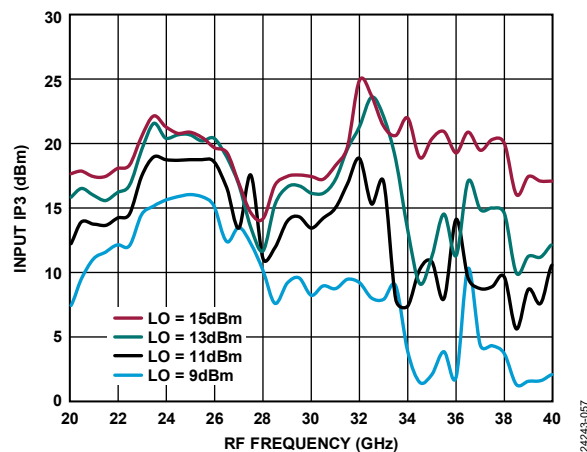
Figure 53. Input IP3 vs. RF Frequency at Various LO Power Levels, TA = 25°C
