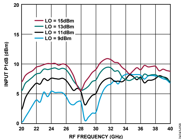
Figure 54. Input P1dB vs. RF Frequency at Various LO Power Levels, TA = 25°C
