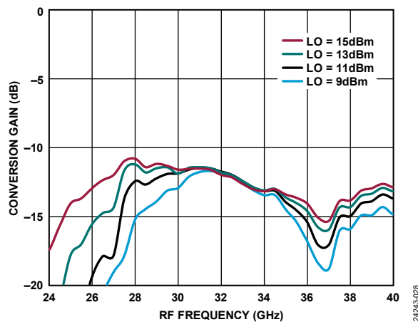
Figure 24. Conversion Gain vs. RF Frequency at Various LO Power Levels, TA = 25°C
