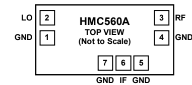
Figure 2. Pad Configuration
