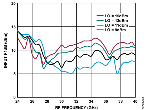
Figure 66. Input P1dB vs. RF Frequency at Various LO Power Levels, TA = 25°C
