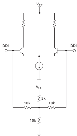
Figure 3-1: Differential Input Stage (DDI/ \overline{\text{DDI}} )
