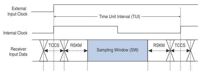
Figure 7-15. High-Speed I/O Timing Diagram
