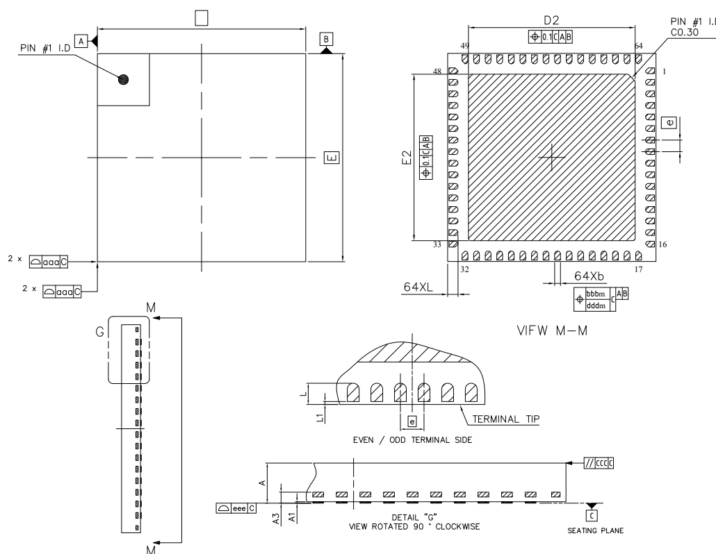
Figure 9.1. QFN64
