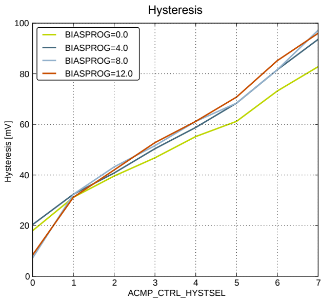
Figure 4.29. ACMP Characteristics, V_{dd} = 3V , Temp = 25^{\circ}C , FULLBIAS = 0 , HALFBIAS = 1
