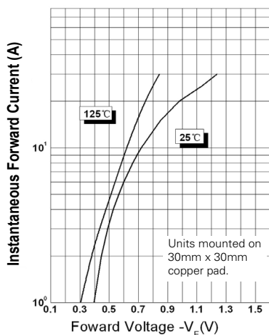
Figure 3: Typical Forward Characteristics
