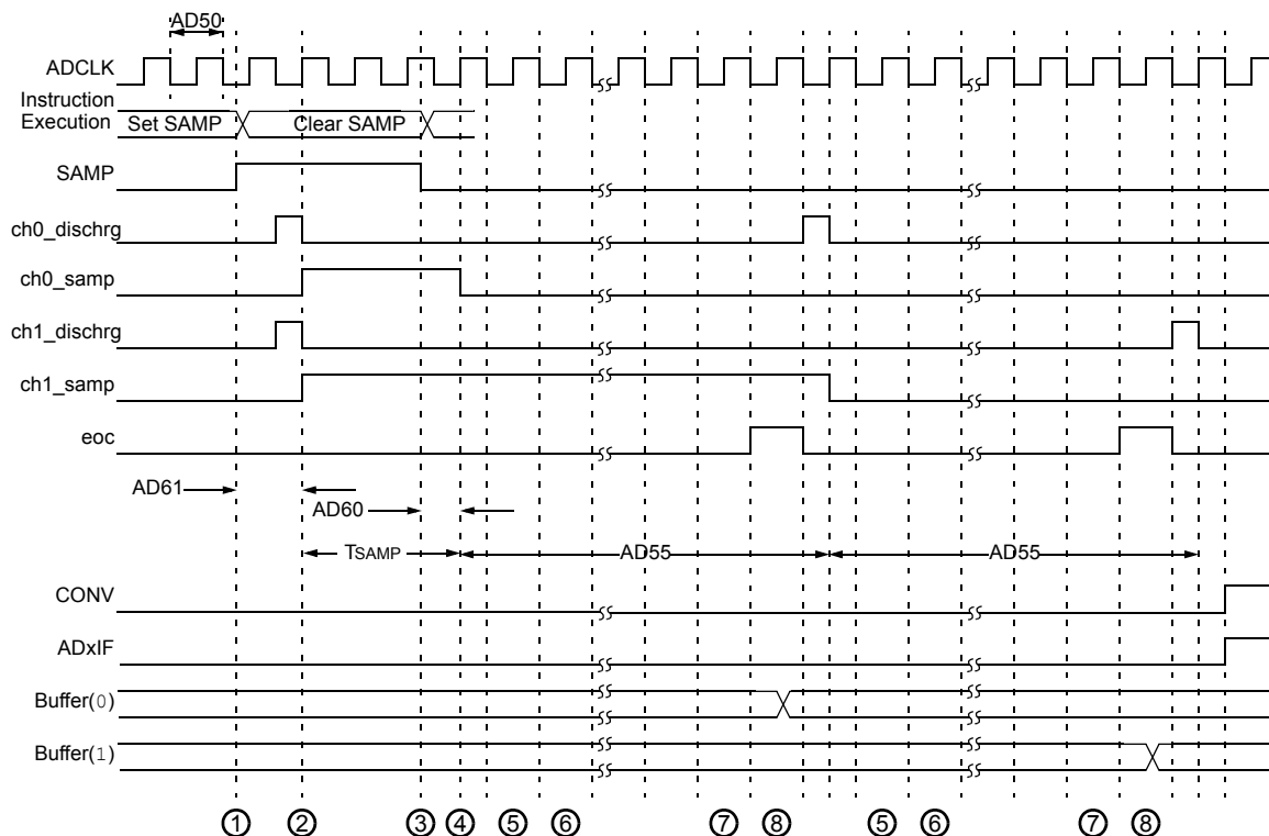
FIGURE 25-25: ADC CONVERSION (10-BIT MODE) TIMING CHARACTERISTICS (CHPS<1:0> = 01, SIMSAM = 0, ASAM = 0, SSRC<2:0> = 000)
