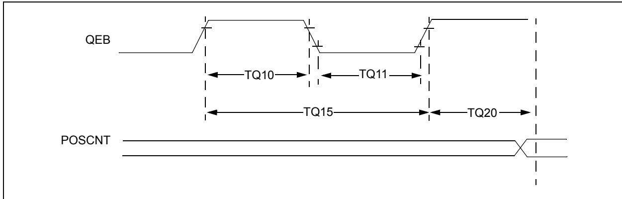
FIGURE 24-8: QE1 MODULE EXTERNAL CLOCK TIMING CHARACTERISTICS
