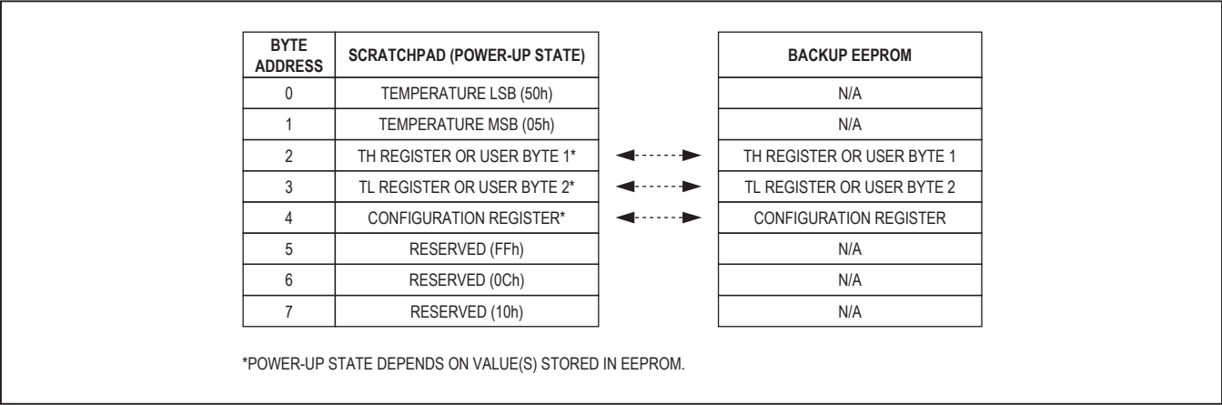
Figure 4. Memory Map
