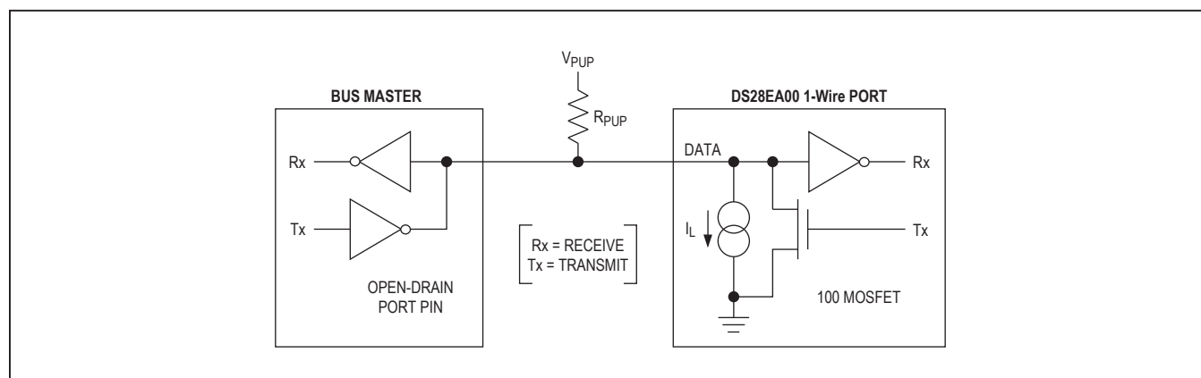
Figure 10. Hardware Configuration
