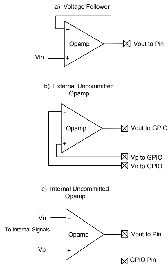
Figure 8-6. Opamp Configurations
