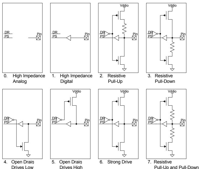
Figure 6-10. Drive Mode
