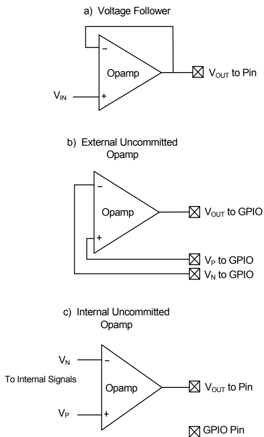
Figure 8-7. Opamp Configurations
