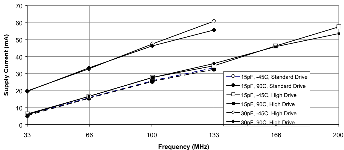
Figure 10. 2.7 V Measured Supply Current versus Frequency, Drive Strength, Loading, and Temperature
