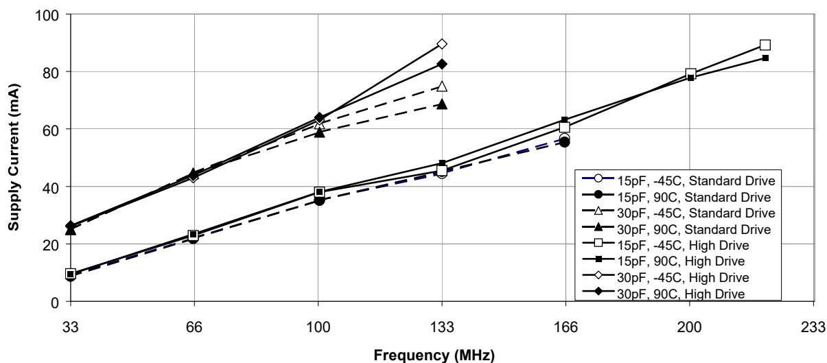
Figure 11. 3.6 V Measured Supply Current versus Frequency, Drive Strength, Loading, and Temperature
