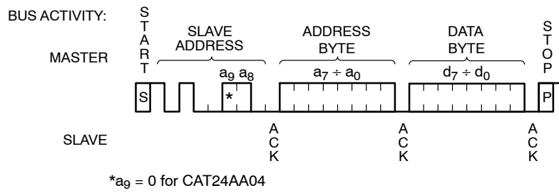
Figure 6. Byte Write Sequence
