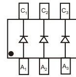
BAT54TW
