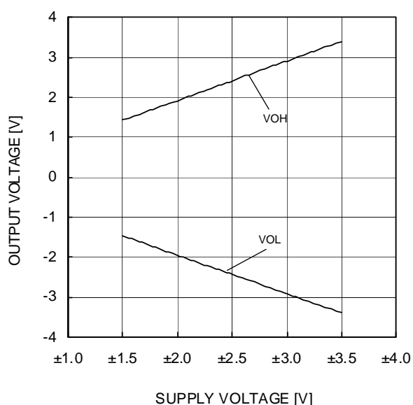
Figure 6. Maximum Output Voltage - Supply Voltage ( R_L=10k\Omega , T_a=25^\circ\text{C} )
