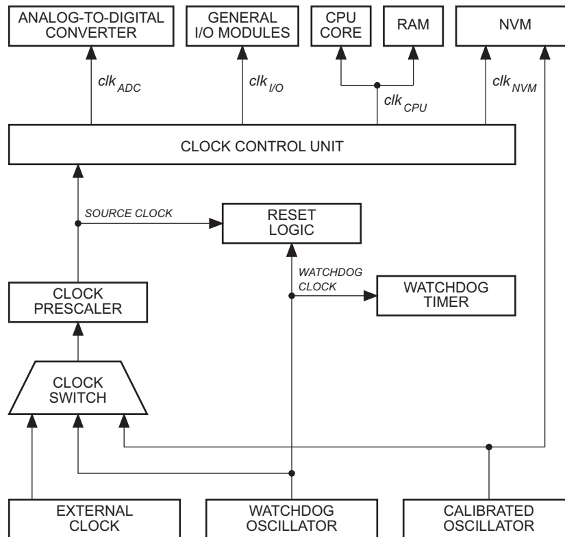
Figure 6-1. Clock Distribution
