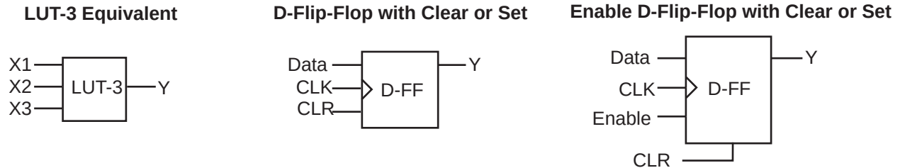
Figure 1-4 • VersaTile Configurations
