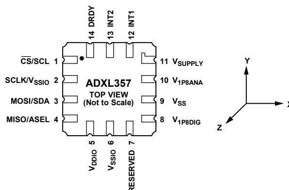
Figure 7. ADXL357 Pin Configuration (SPI/I²C)
