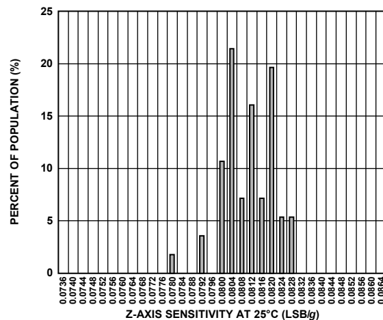
Figure 25. ADXL356 Sensitivity Histogram at 25°C, Z-Axis
