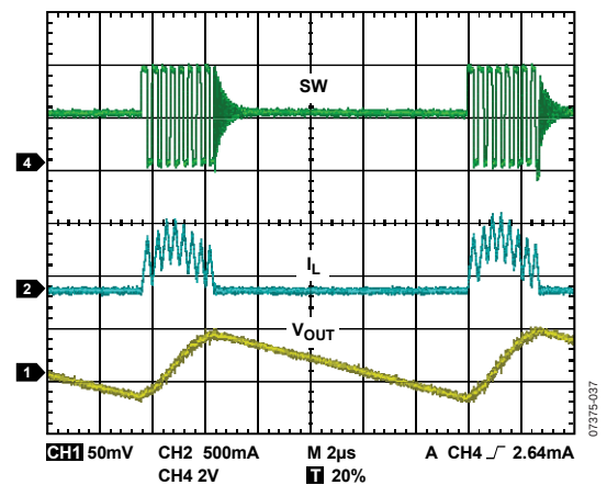
Figure 27. Typical Power Save Mode Waveform, 50 mA
