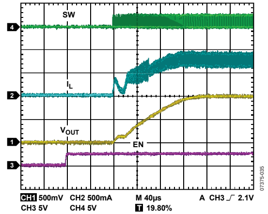
Figure 25. Start-Up, V_{OUT} = 1.0\text{ V} , 600 mA
