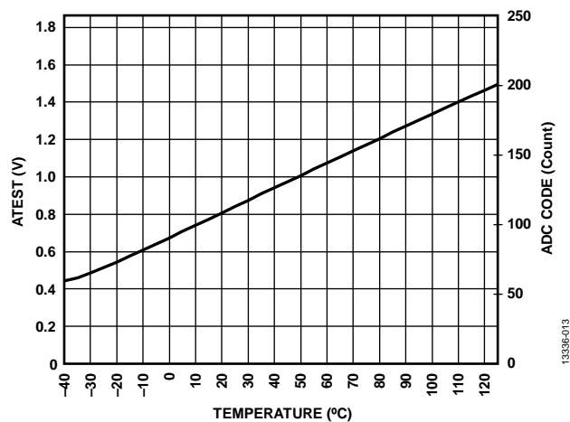
Figure 13. ATEST Voltage and ADC Code vs. Temperature
