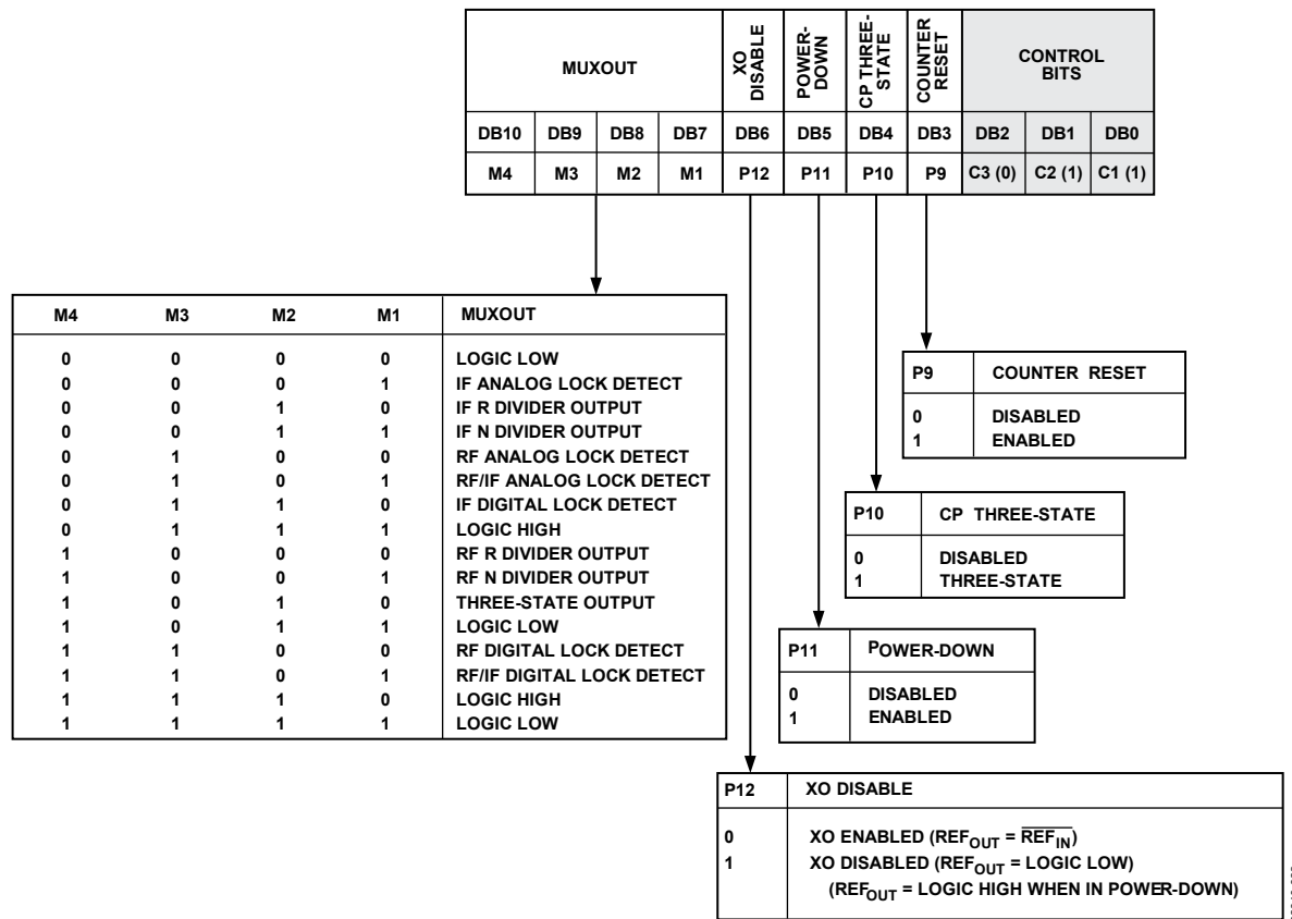
Figure 38. Master Register Map
