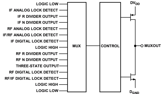
Figure 33. MUXOUT Circuit
