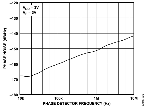
Figure 25. Phase Noise (Referred to CP Output) vs. PFD Frequency, IF Side
