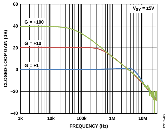
Figure 40. Closed-Loop Gain vs. Frequency, V_{SY} = \pm 5V
