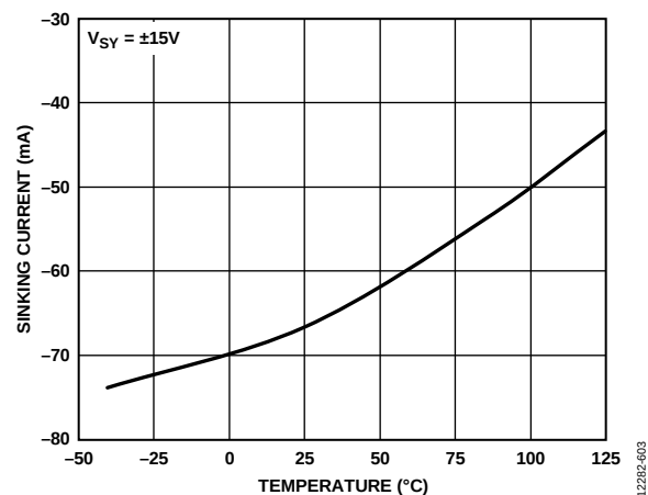
Figure 83. Output Short-Circuit Sinking Current vs. Temperature, V_{SY} = \pm 15\text{ V}
