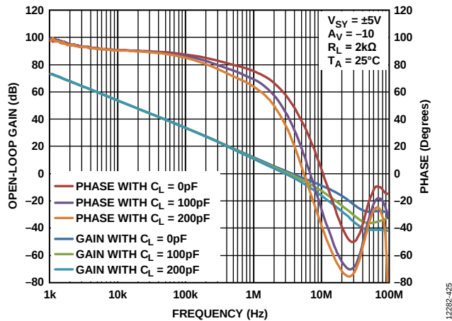
Figure 39. Open-Loop Gain and Phase vs. Frequency, V_{SY} = \pm 5V
