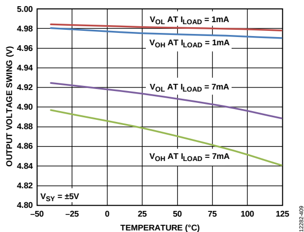
Figure 27. Output Voltage Swing vs. Temperature, V_{SY} = \pm 5V
