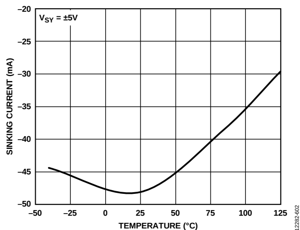
Figure 81. Output Short-Circuit Sinking Current vs. Temperature, V_{SY} = \pm 5\text{ V}
