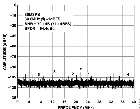
Figure 7. AD9629-80 Single-Tone FFT with f_{IN} = 30.6 MHz
