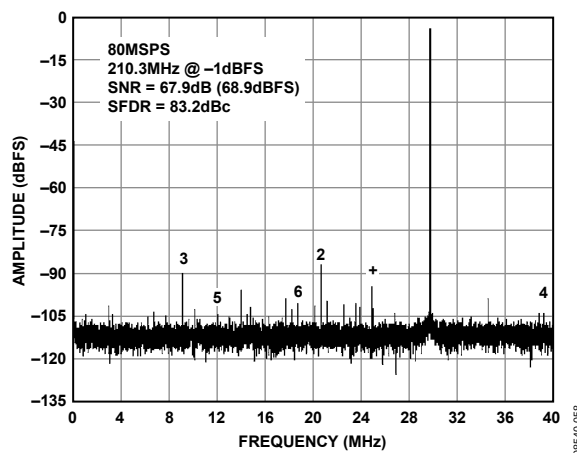
Figure 8. AD9629-80 Single-Tone FFT with f_{IN} = 210.3 MHz
