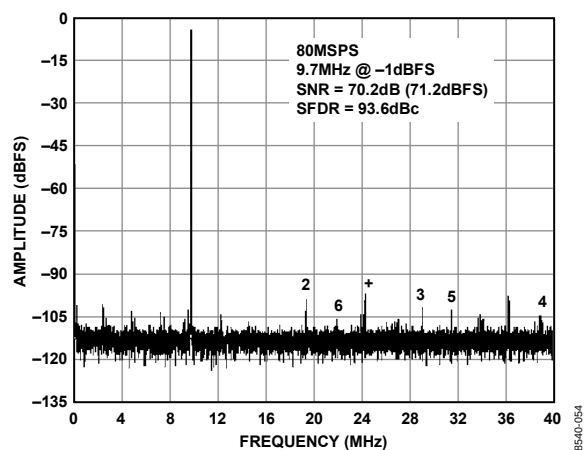
Figure 4. AD9629-80 Single-Tone FFT with f_{IN} = 9.7 MHz
