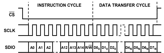
Figure 88. Serial Register Interface Timing, LSB First, Register 0x000, Bit 5 and Bit 2 = 1
