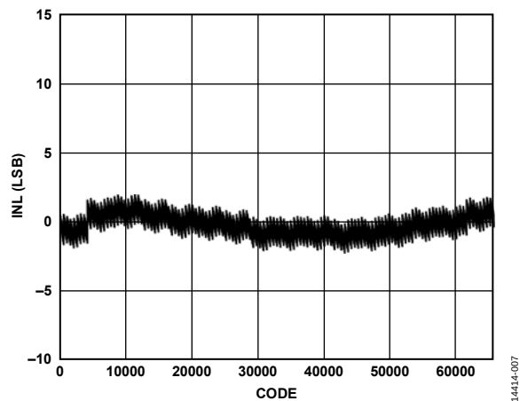
Figure 8. INL, I_{OUTFS} = 40\text{ mA}
