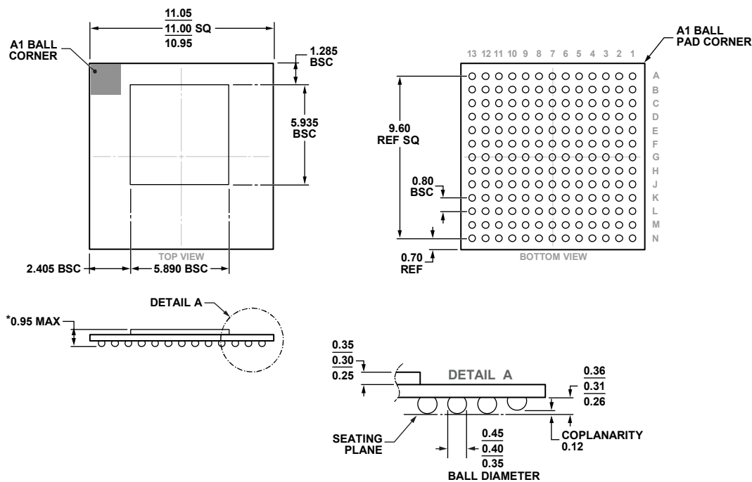
Figure 144. 169-Ball Chip Scale Package Ball Grid Array [CSP_BGA] (BC-169-2) Dimensions shown in millimeters
