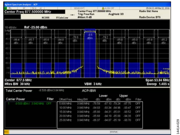
Figure 32. Single-Carrier W-CDMA at 877.5 MHz
