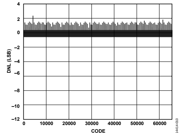
Figure 11. DNL, I_{OUTFS} = 40\text{ mA}
