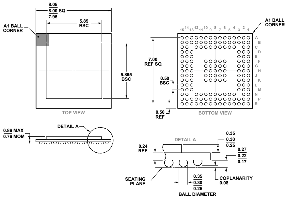
Figure 143. 165-Ball Chip Scale Package Ball Grid Array [CSP_BGA] (BC-165-1) Dimensions shown in millimeters
