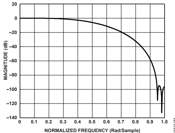
Figure 118. Fourth 2x Half-Band 11.25% Filter Response
