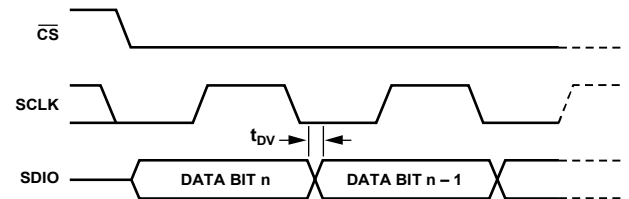
Figure 89. Timing Diagram for Serial Port Register Read
