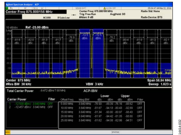
Figure 35. Two-Carrier W-CDMA at 875 MHz
