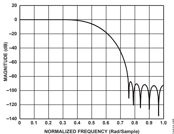
Figure 119. FIR85 2x Half-Band 45% Filter Response
