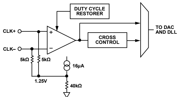
Figure 133. Clock Input
