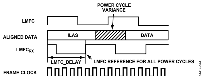
Figure 104. LMFC_DELAY_x to Compensate for Link Delay &gt; LMFC
