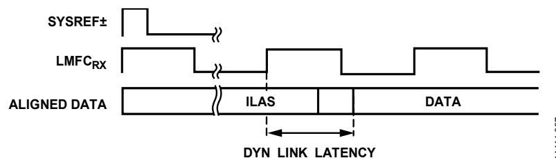
Figure 106. DYN_LINK_LATENCY_x Illustration
