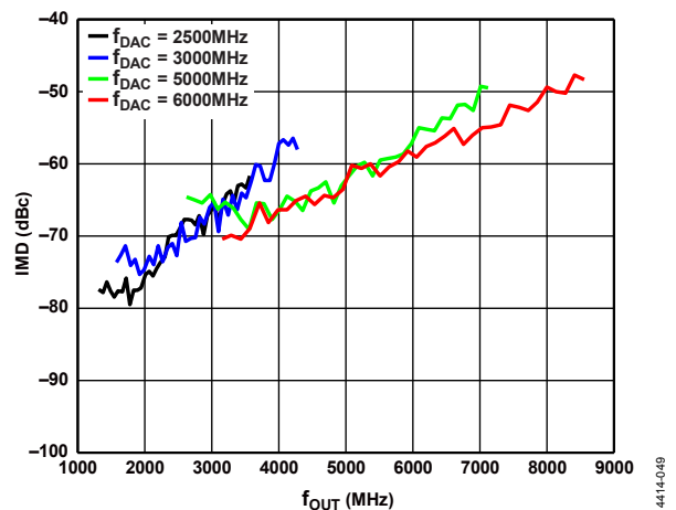
Figure 53. IMD vs. f_{OUT} over f_{DAC}
