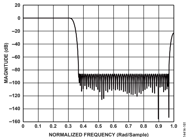
Figure 115. 3x Third-Band 90% Filter Response
