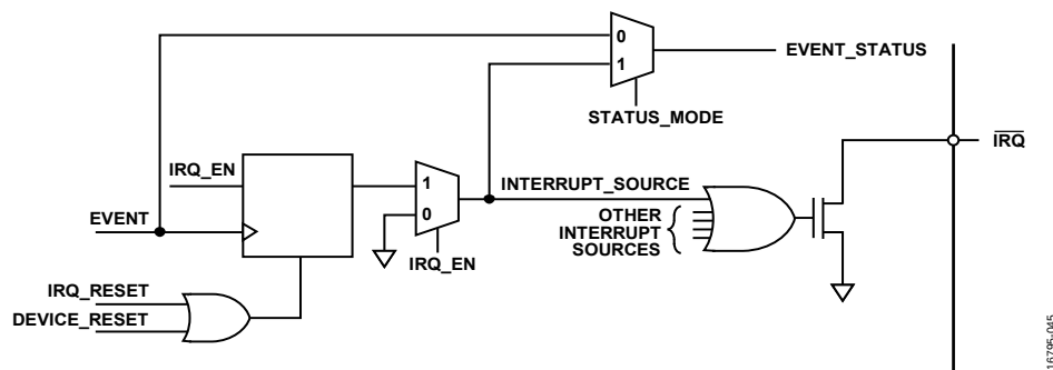
Figure 89. Simplified Schematic of \overline{IRQx} Circuitry
