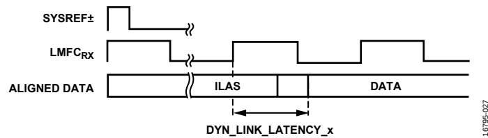
Figure 69. DYN_LINK_LATENCY_x Illustration
