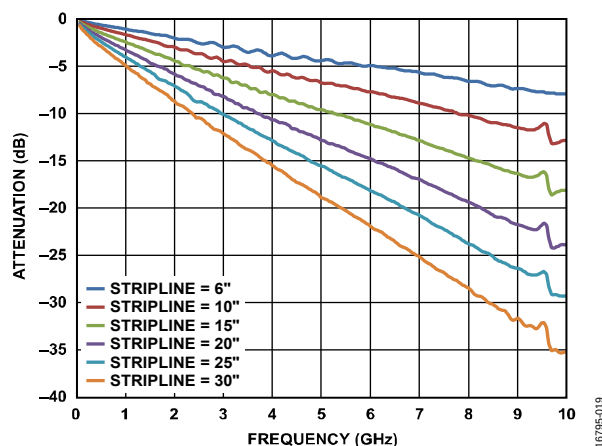
Figure 59. Insertion Loss of 50 \Omega Striplines on FR4
