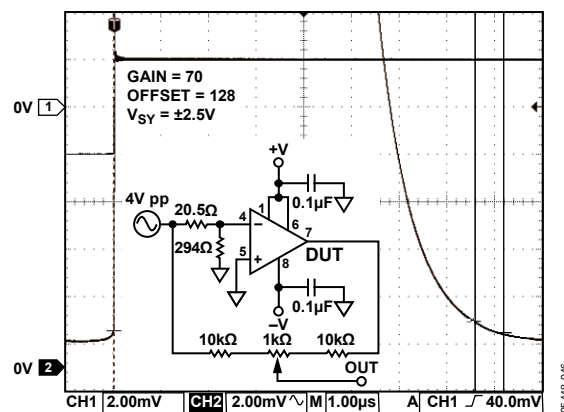
Figure 45. Settling Time 0.01%
