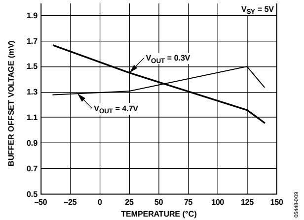
Figure 8. Output Buffer Offset Voltage vs. Temperature
