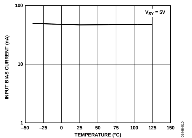
Figure 9. Input Bias Current at V_{POS} , V_{NEG} vs. Temperature
