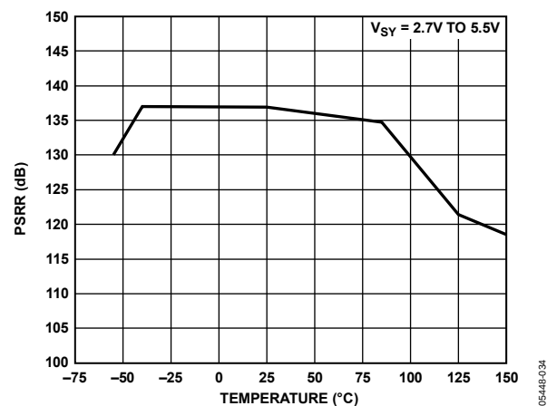
Figure 33. PSRR vs. Temperature
