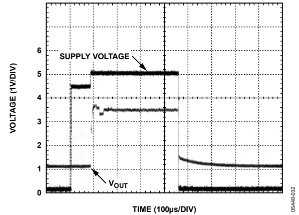
Figure 31. Power-On Response at 125°C
