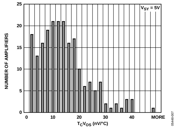
Figure 7. T_cV_{os} at V_{SY} = 5V
