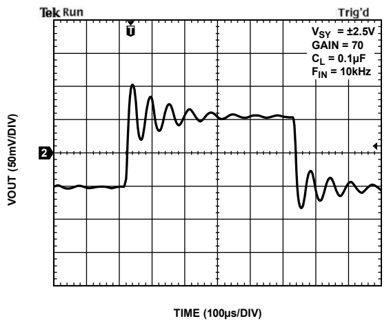
Figure 35. Small Signal Response at C_L = 0.1 \mu F and F_{IN} = 10 \text{ kHz}
