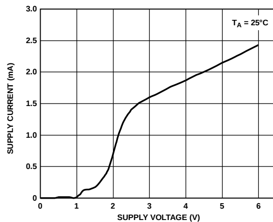
Figure 14. Supply Current ( I_{SV} ) vs. Supply Voltage
