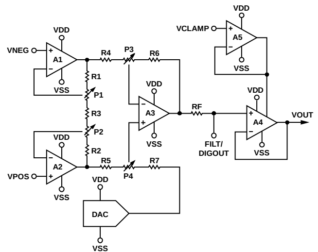
Figure 47. Functional Schematic
