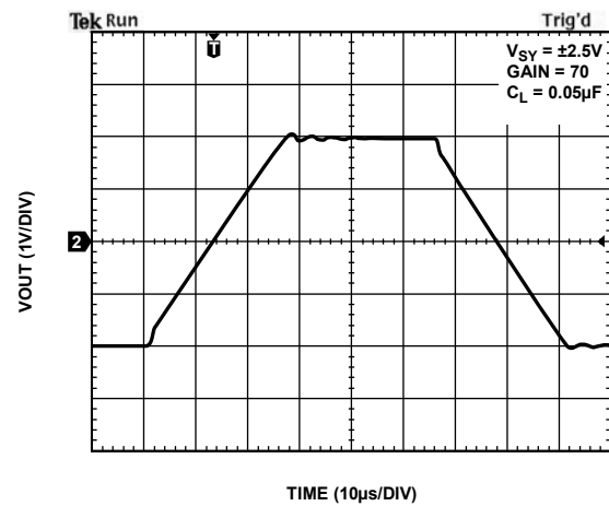
Figure 38. Large Signal Response at C_L = 0.05 \mu F
