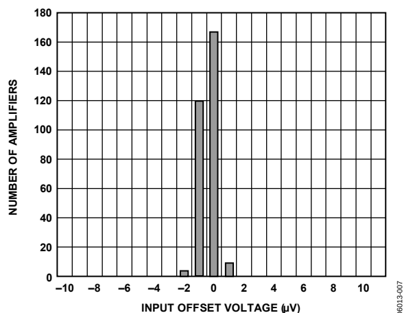
Figure 7. Input Offset Voltage Distribution, V_{SY} = 2.7V
