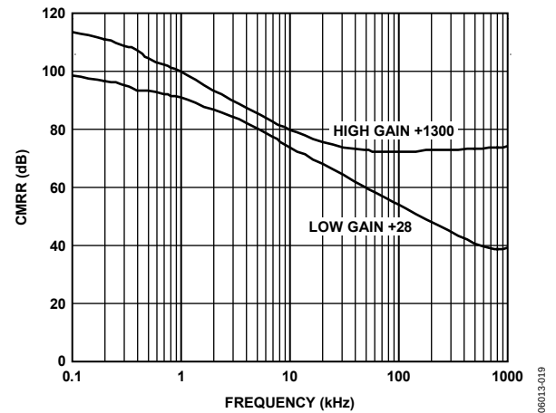
Figure 19. CMRR vs. Frequency, V_{SY} = 5\text{ V}
