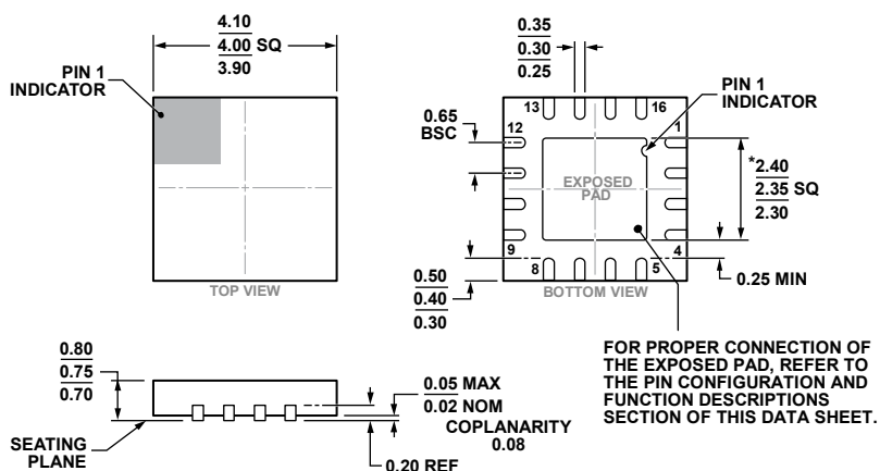
Figure 49. 16-Lead Lead Frame Chip Scale Package [LFCSP] 4 mm × 4 mm Body and 0.75 mm Package Height (CP-16-20)
