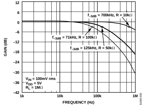
Figure 30. -3 dB Bandwidths
