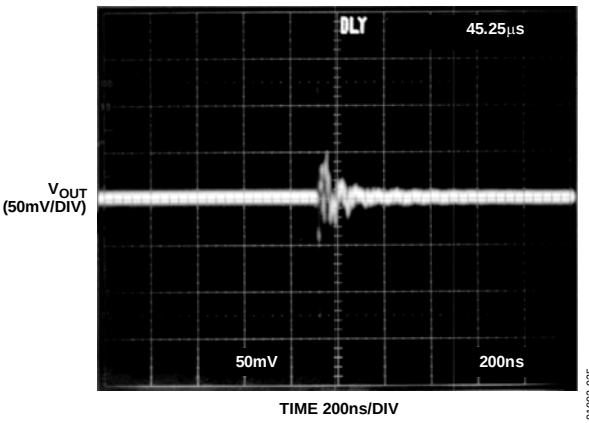
Figure 25. Digital Feedthrough vs. Time
